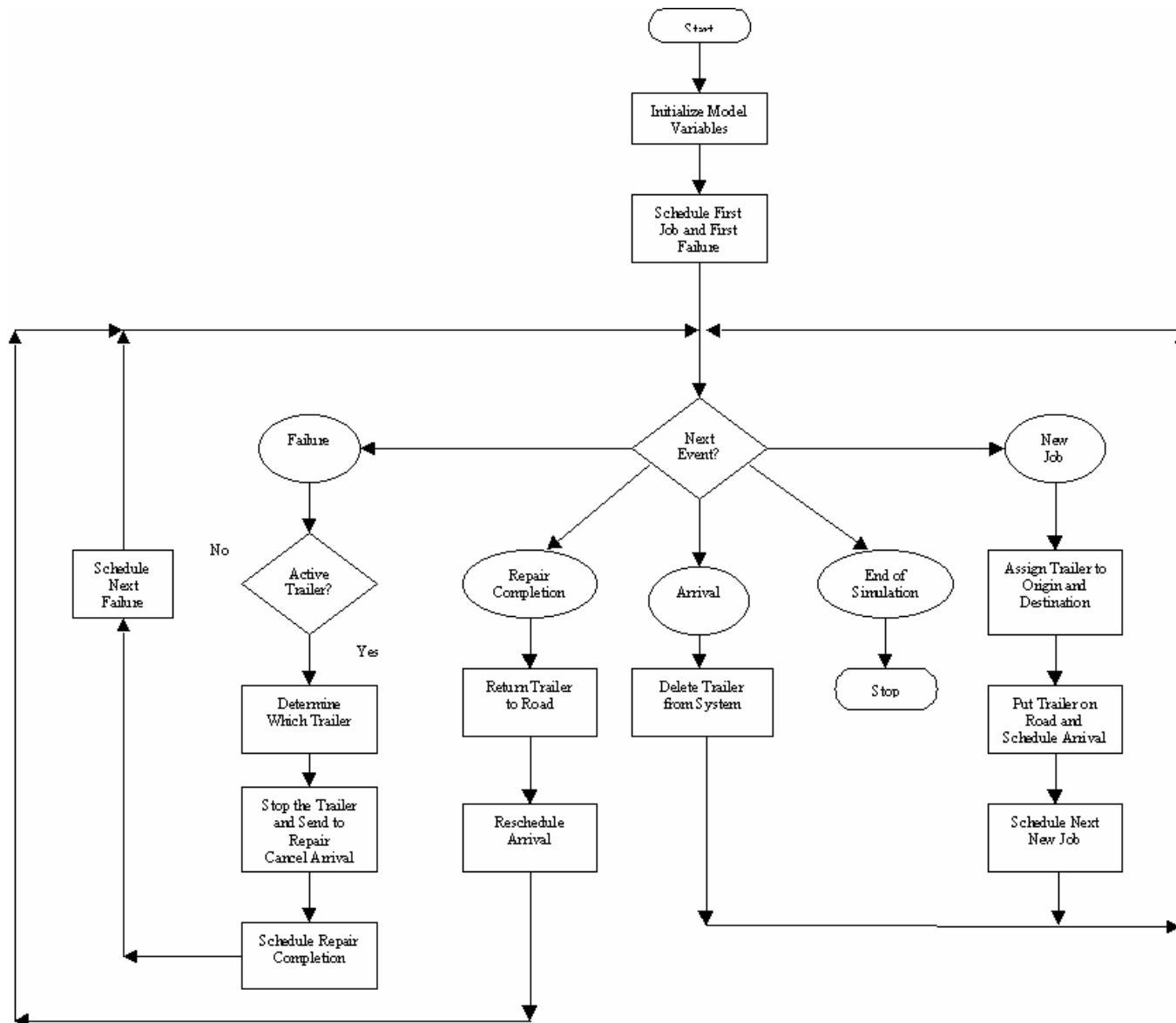
Figure 11. Flowchart showing simulation logic excluding data collection and output.
