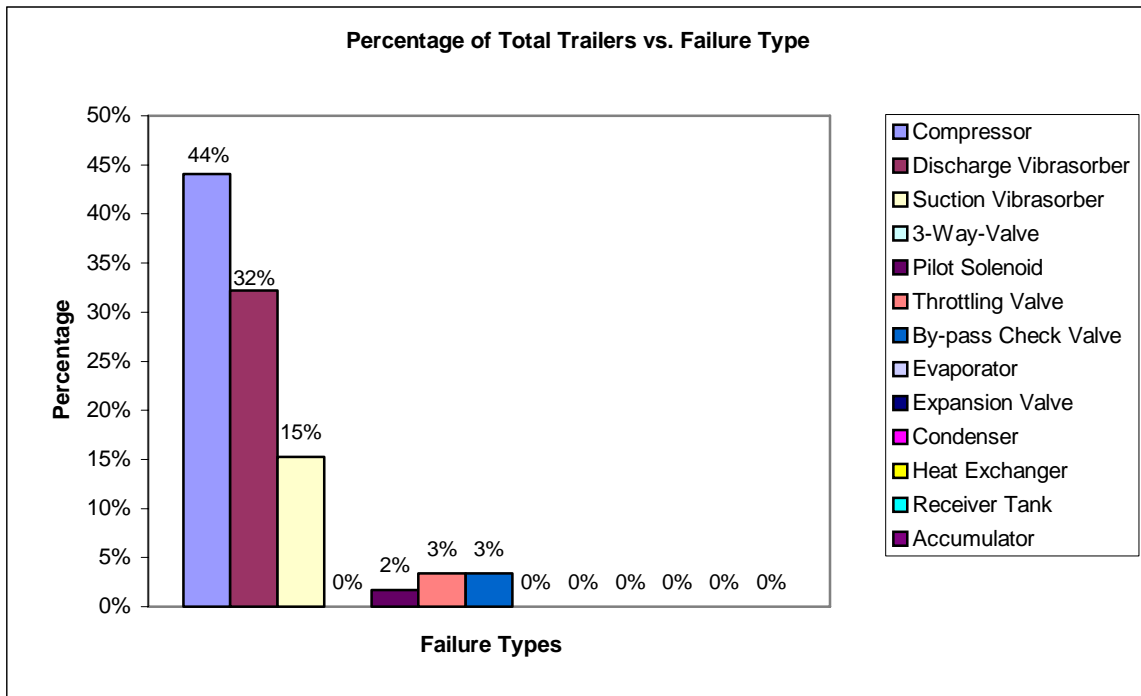
Figure 9. 1994 Trailers Pareto Analysis.
