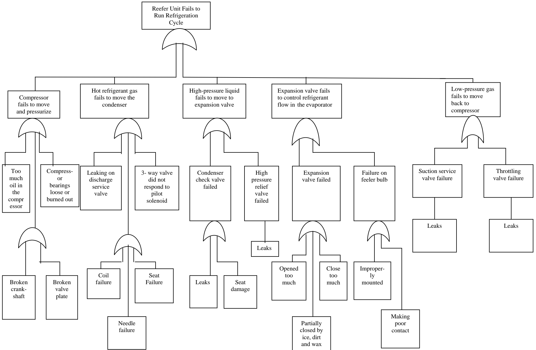
Figure 3. Fault Tree Analysis – Refrigeration Cycle (Thermo King).
