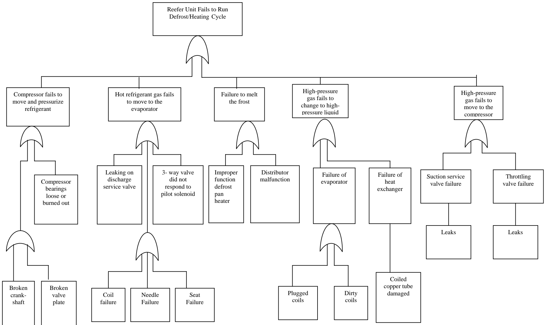
Figure 4. Fault Tree Analysis – Heating/Defrost Cycle (Thermo King).
