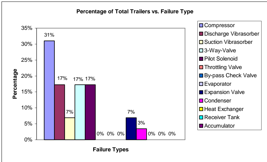
Figure 10. 1995 Trailers Pareto Analysis.
