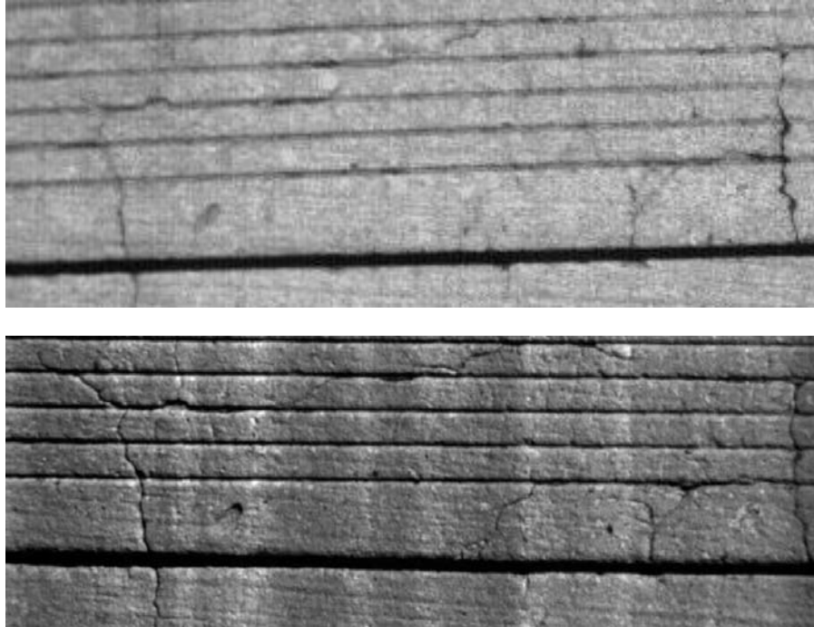
Figure 6 Distresses of Zoomed-in Area from Figure 5
